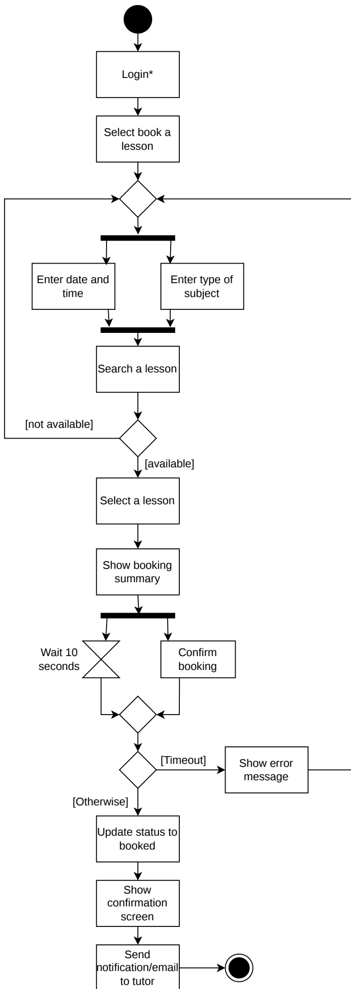
Activity Diagram: Book a lesson
