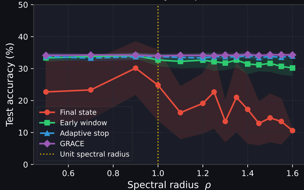
CIFAR-10: Accuracy vs Spectral Radius
