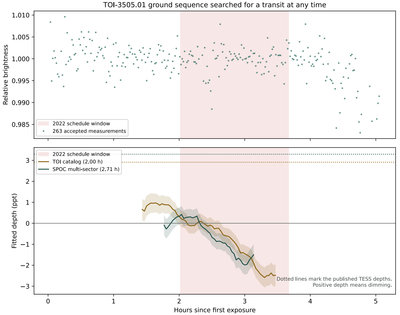
Figure 5. Whole-sequence transit search. Top: the 263 accepted measurements, with the 2022 schedule window shaded. Bottom: fitted depth against trial midpoint for the catalog and SPOC durations, with one-sigma bands; dotted lines mark the published TESS depths. Positive depth denotes dimming. The scan is restricted to midpoints where the event is well sampled with baseline on both sides, so it does not extend to the ends of the night.
