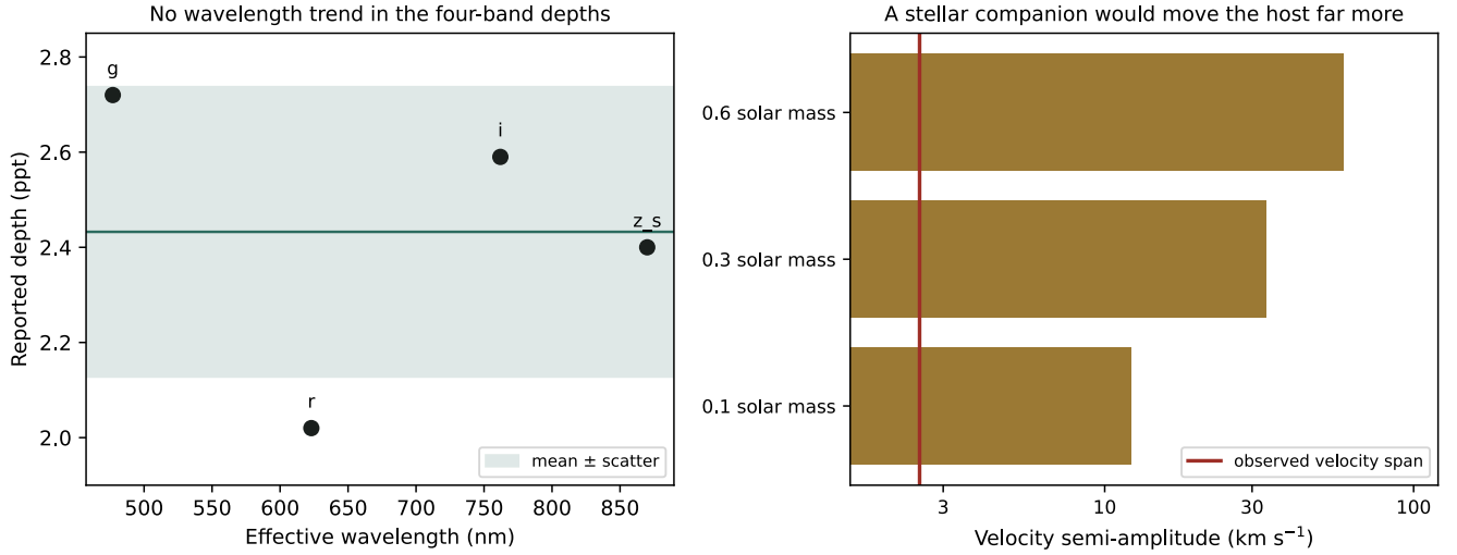
Figure 6. False-positive scenario tests. Left: the four reported MuSCAT2 depths against effective wavelength, with the mean and its scatter shaded; a blended eclipsing binary would generally produce a trend. Right: circular, edge-on velocity semi-amplitudes for stellar companions at the adopted period, against the span of the three public reconnaissance velocities. Both use published values and are not re-reductions.
