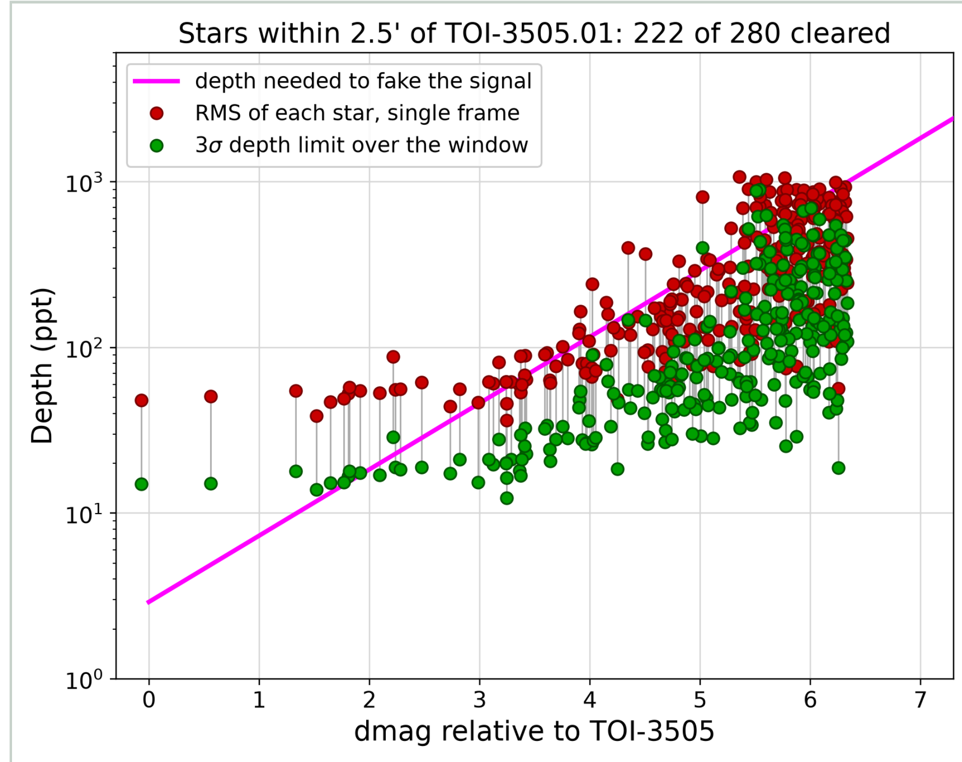
Fig. 5. Each neighbour's brightness difference against how deep we can see. The magenta line is the eclipse depth that star would need to fake our signal. Red is the scatter in a single frame, green is the depth limit after using the whole window, and the grey bars connect the same star. Green points below the line are cleared.
