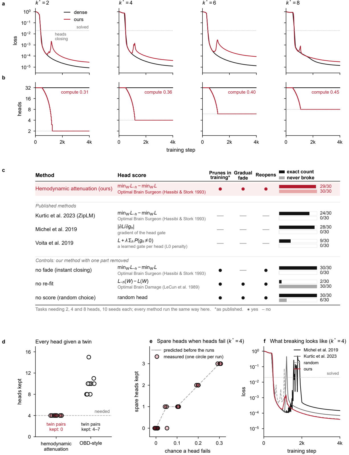
Figure 2: Hemodynamic attenuation during training. a , Loss of the dense model (black) and with hemodynamic attenuation (red) for k^* = 2, 4, 6, 8 (one seed each); dotted line, the solved bar. The small rise is heads fading out. b , Number of open heads; dotted line, k^* . “Compute” is head-steps used, as a fraction of the dense model’s, including the cost of valuing heads. c , Every method on the same 30 runs ( k^* = 2, 4, 8, 10 seeds each), all run the same way here: how it scores a head, whether it prunes during training as published, fades heads gradually, and can reopen them, and how often it kept exactly k^* heads (dark bar) and never broke the model (light bar). Published
