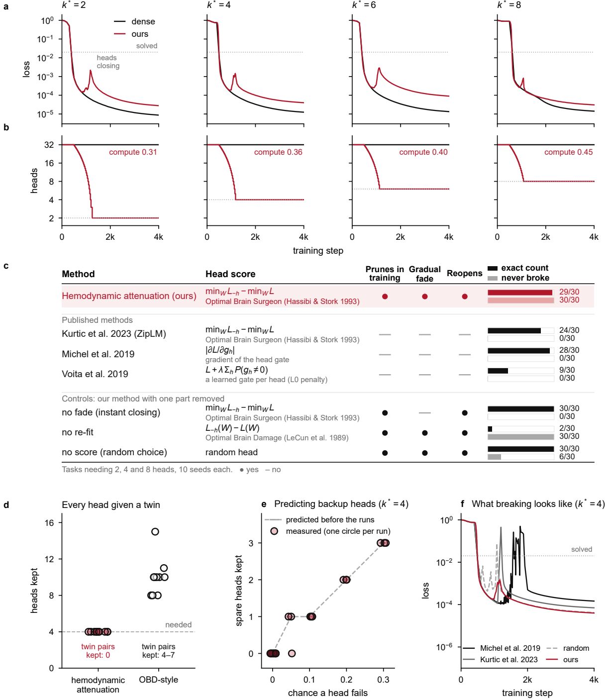
Figure 2: Hemodynamic attenuation during training. a , Loss of the dense model (black) and with hemodynamic attenuation (red) for k^* = 2, 4, 6, 8 (one seed each); dotted line, the solved bar. The small rise is heads fading out. b , Number of open heads; dotted line, k^* . “Compute” is head-steps used, as a fraction of the dense model’s, including the cost of valuing heads. c , Every method on the same 30 runs ( k^* = 2, 4, 8, 10 seeds each), all run the same way here: how it scores a head, whether it prunes during training as published, fades heads gradually, and can reopen them, and how often it kept exactly k^* heads (dark bar) and never broke the model (light bar). Published methods above; below, controls that remove one part of our method. d , Runs that start with every head copied ( k^* = 4 , 10 runs each; one circle per run): heads kept, and how many twin pairs kept both copies. e , Spare heads kept when each head fails with chance p at every step ( k^* = 4 ): one circle per run (10 runs at p = 0 , 3 at each other p ), against the number predicted before the runs (dashed). f , One run of each method ( k^* = 4 , seed 0): only hemodynamic attenuation stays below
