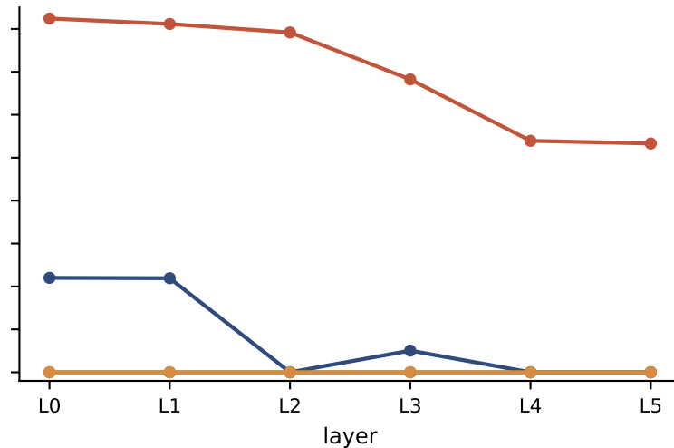
Inception1d
