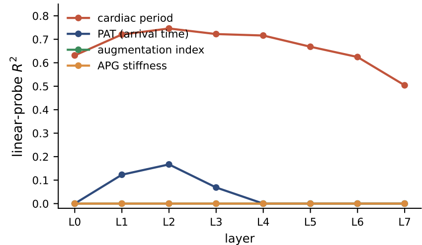
XResNet50
