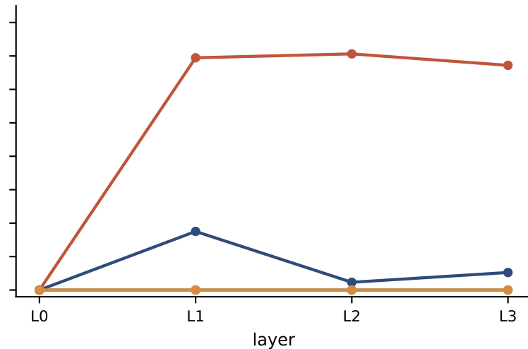
Transformer
