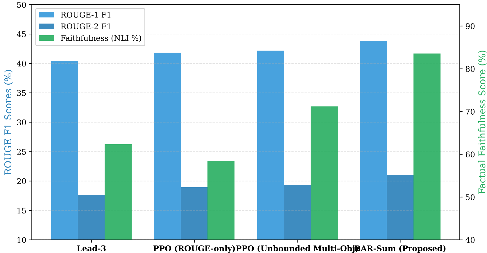
Performance and Factual Adherence Across Model Baselines
