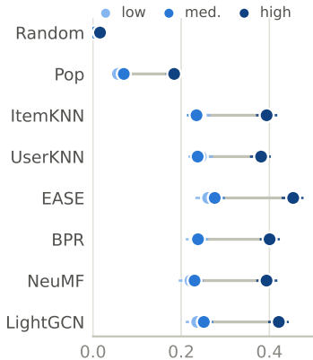
(a) NDCG@10, user activity
