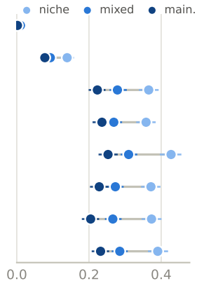
(c) NDCG@10, user taste
