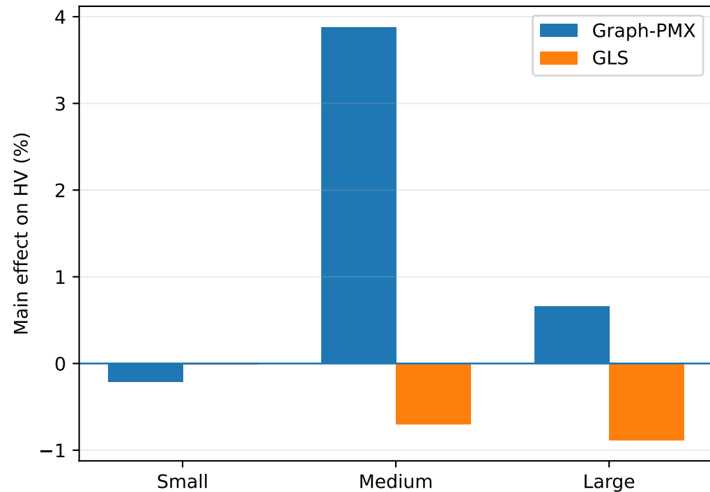
Hypervolume
