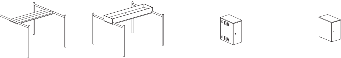
Top fonoassorbente - Sound-absorbing top 140 / 160 / 180 x 148 x 100h. cm Top portapiante - Plant holder top 140 / 160 / 180 x 148 x 111h. cm Porta CPU - CPU holder 40 x 70 x 74h. cm Mobile con anta - Side cabinet with door 40 x 70 x 74h. cm
