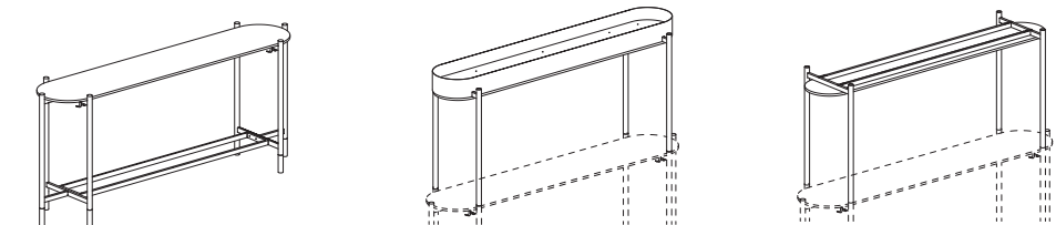
Tavolo - Table 158 x 58 x 111h. cm Top portapiante - Plant holder top 138 x 58 x 111h. cm Top fonoassorbente - Sound absorbing top 138 x 58 x 100h. cm
