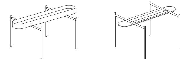
Top portapiante - Plant holder top 160 x 128 x 111h. cm 200 x 148 x 111h. cm Top fonoassorbente - Sound absorbing top 160 x 128 x 100h. cm 200 x 148 x 100h. cm
