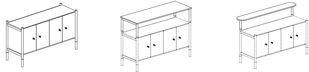
Mobile laterale - Sideboard 148 x 52 x 74h. cm Mensola per mobile laterale - Shelf for sideboard 149 x 53 x 35h. cm Top counter per mobile laterale - Top counter for sideboard 158 x 24 x 24h. cm
