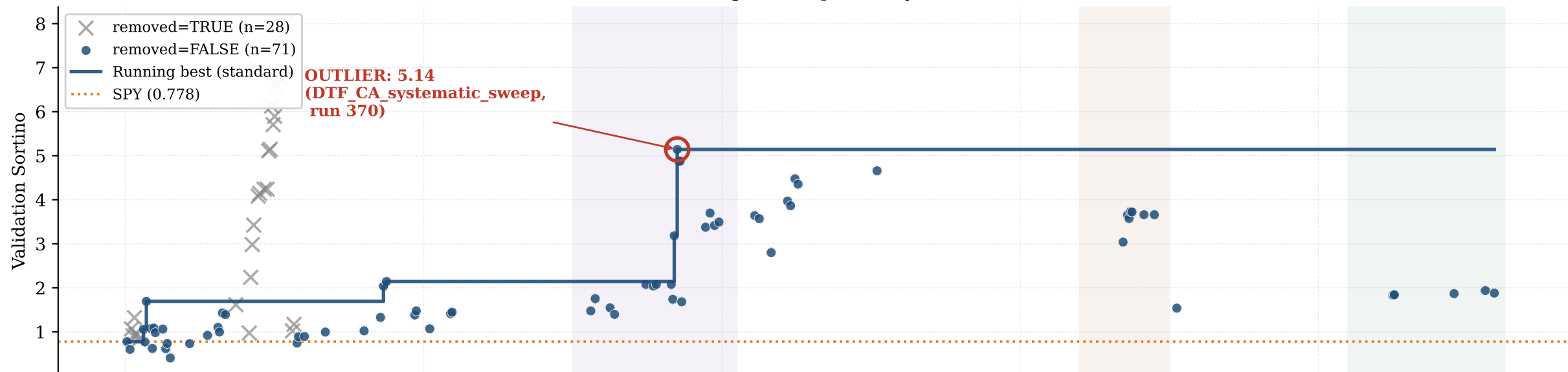
Sortino: standard running-best — pinned by outlier 5.14 at run 370
