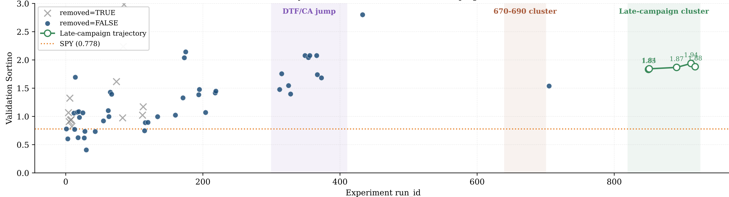
Sortino: y-axis zoomed to (0, 3.0) — late-campaign view
