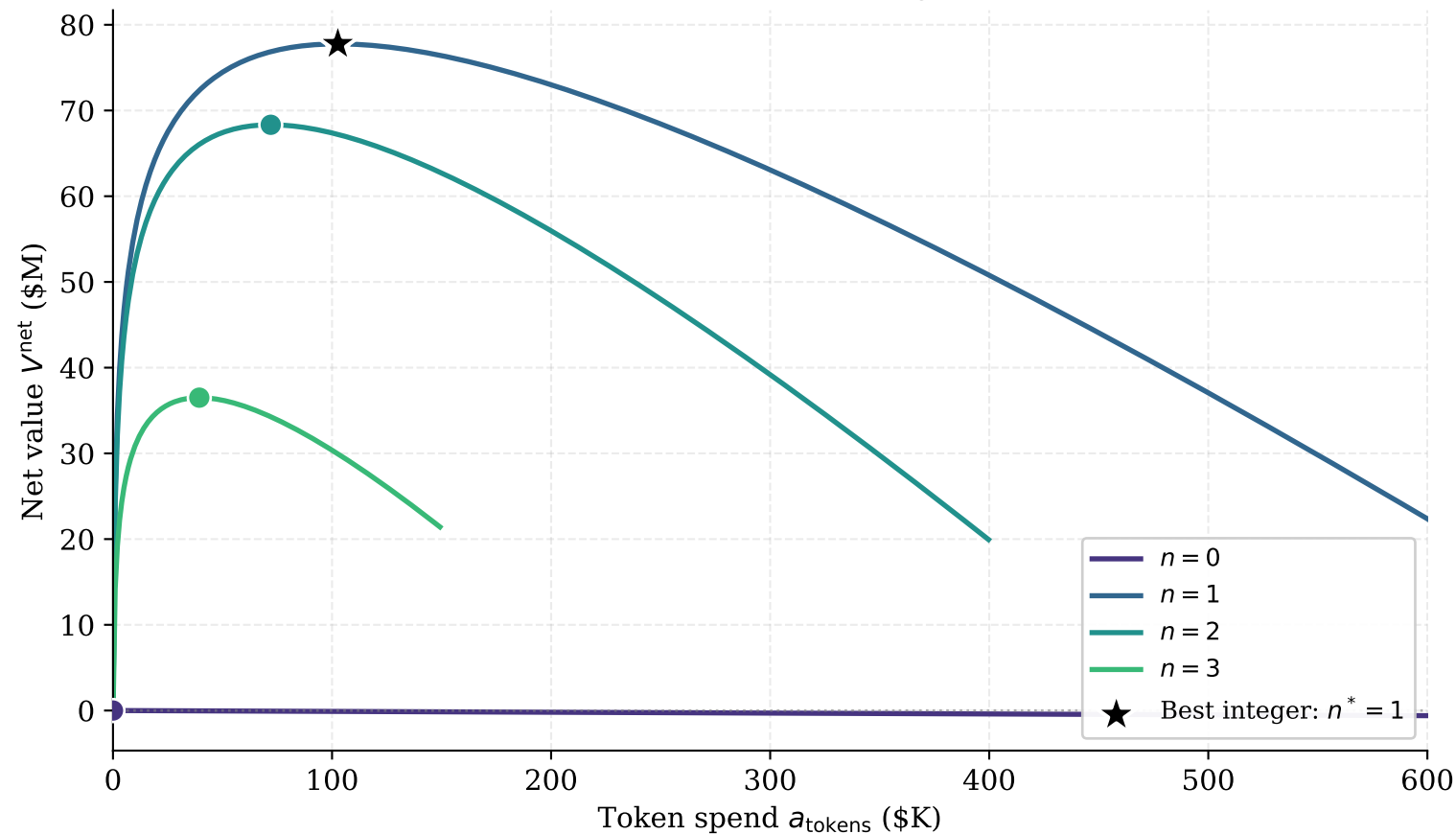
(a) V^{\text{net}}(n, a) for each integer n
