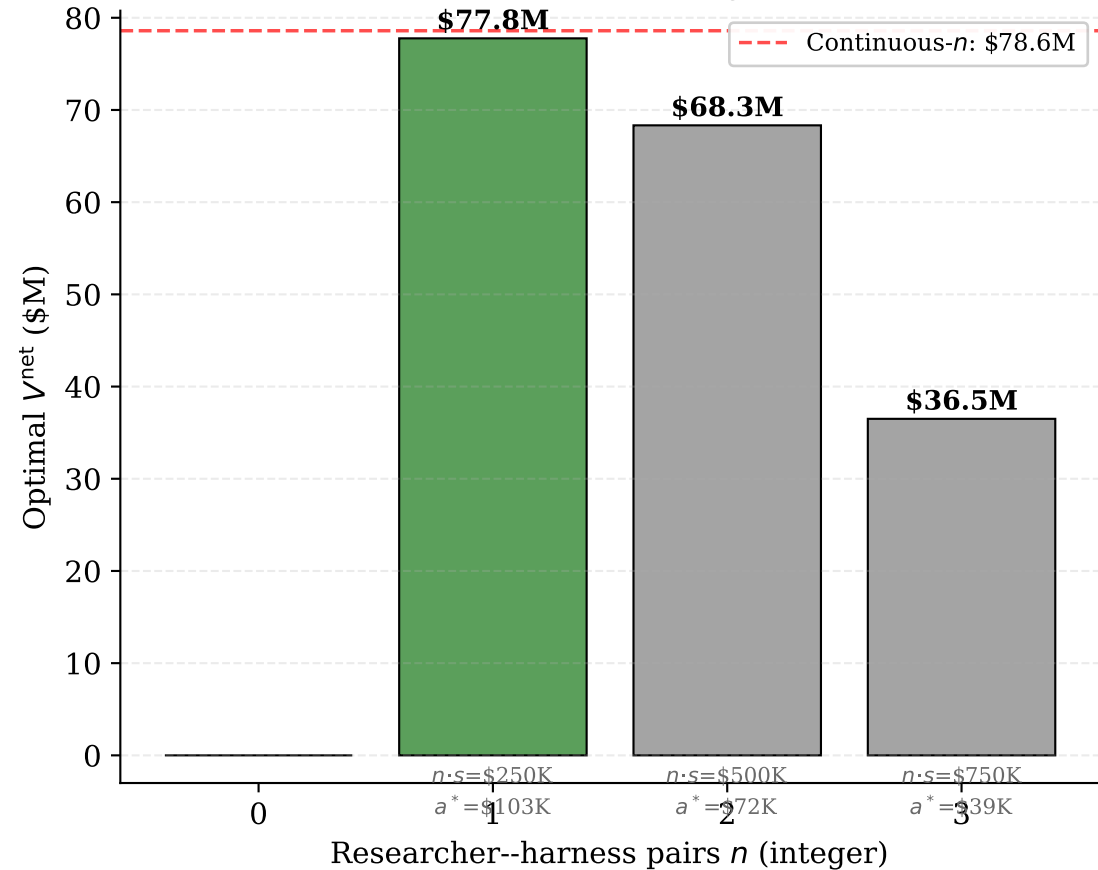
(b) Best V^{\text{net}} per integer n
