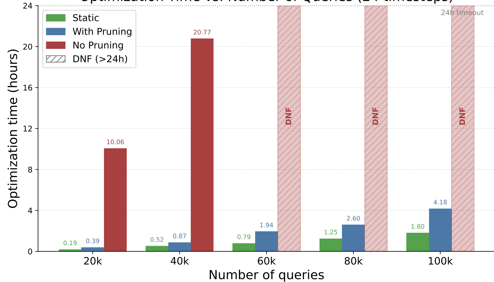
Optimization Time vs. Number of Queries (24 timesteps)
