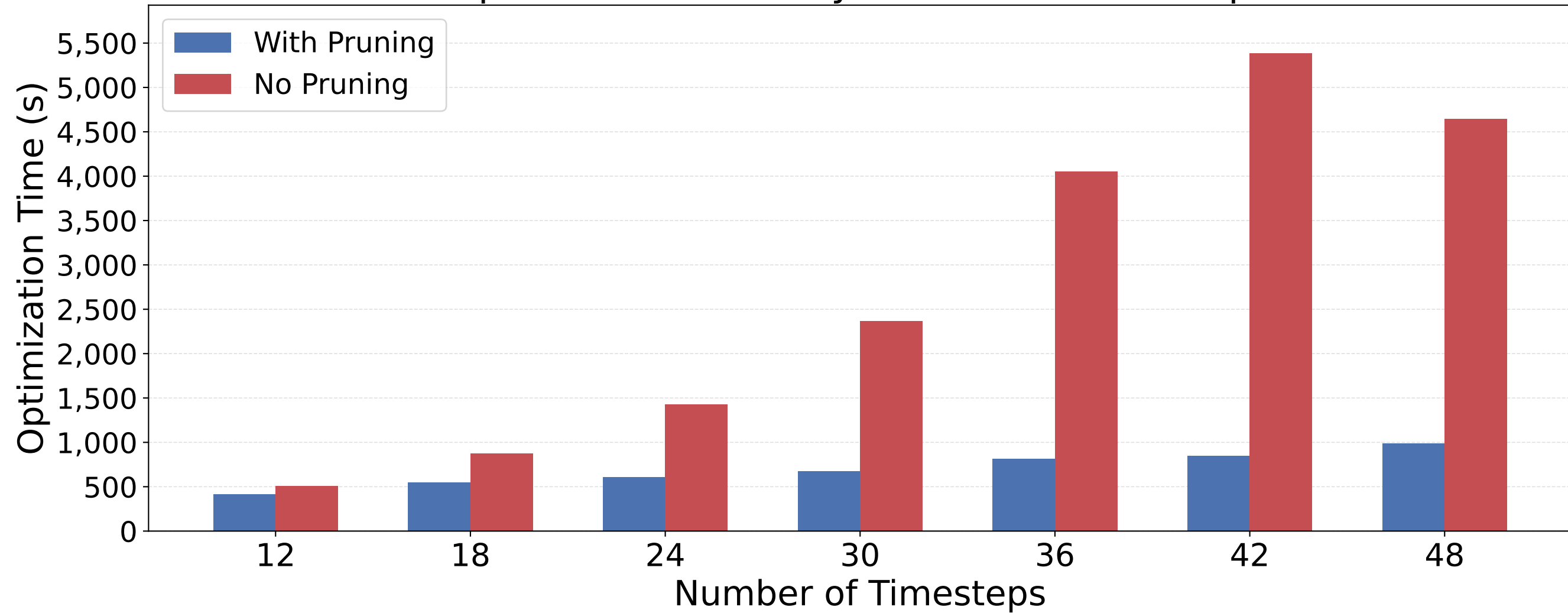
Optimization Time by Number of Timesteps
