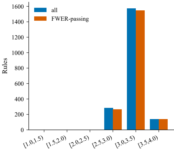
ABIDE: rule count per lift band
