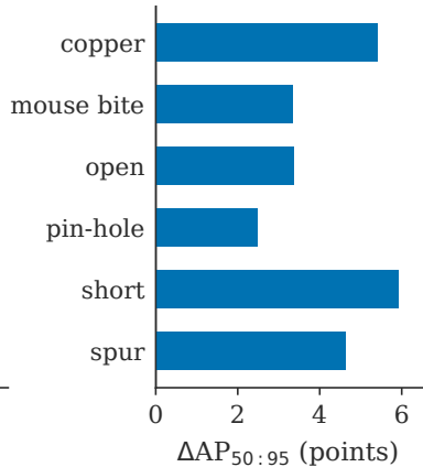
(c) DeepPCB classes
