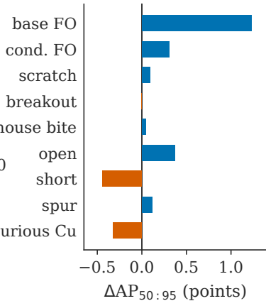
(b) DsPCBSD+ classes
