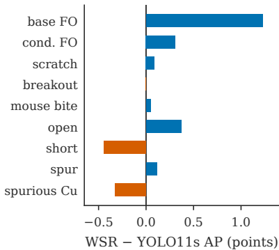
(b) DsPCBSD+ classes
