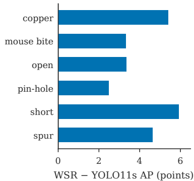
(c) DeepPCB classes
