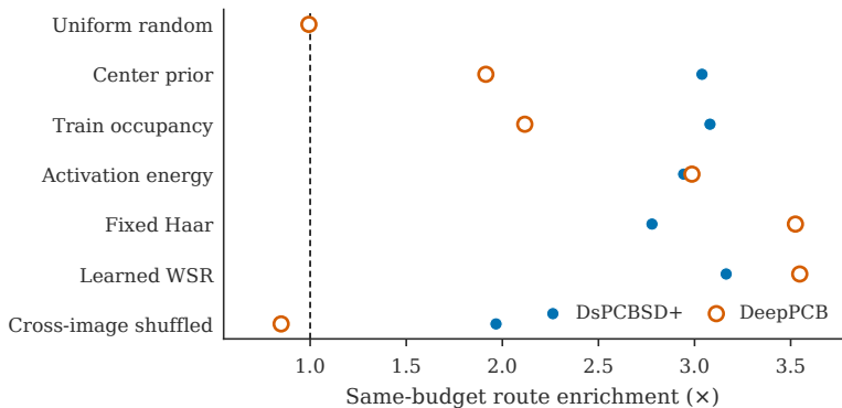
(b) Same-budget route controls
