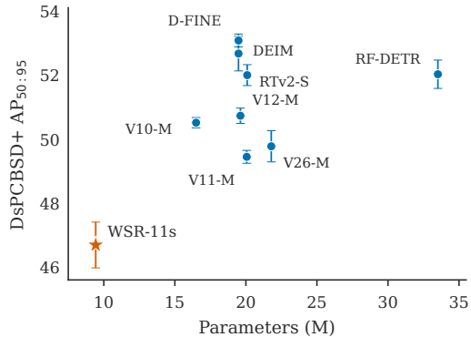
(a) Accuracy-size context
