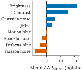
(a) Corruption effect
