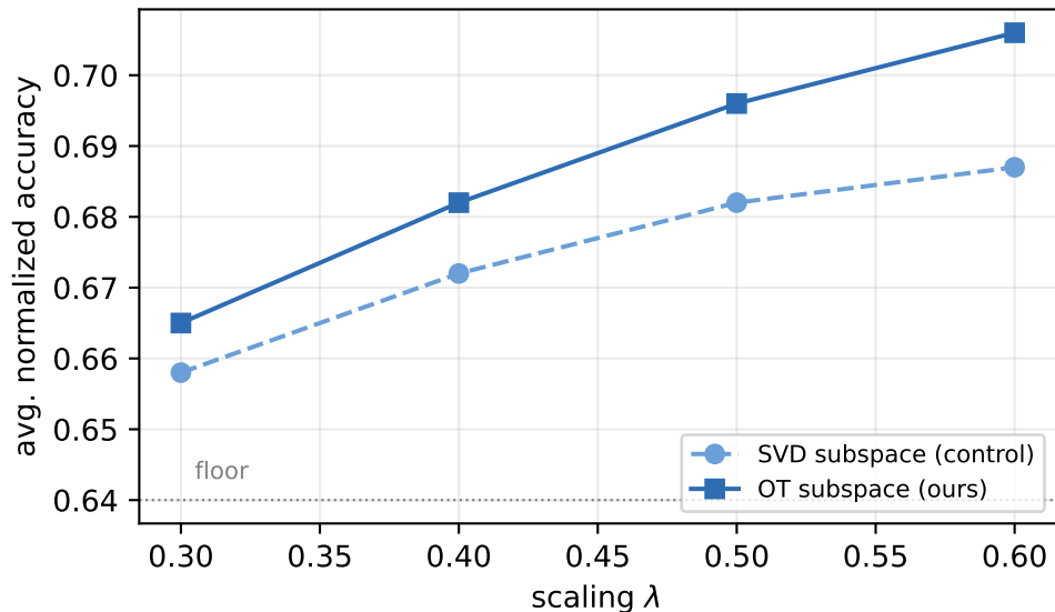
OT subspace beats SVD at every \lambda (identical TIES, \kappa = 0.2 )
