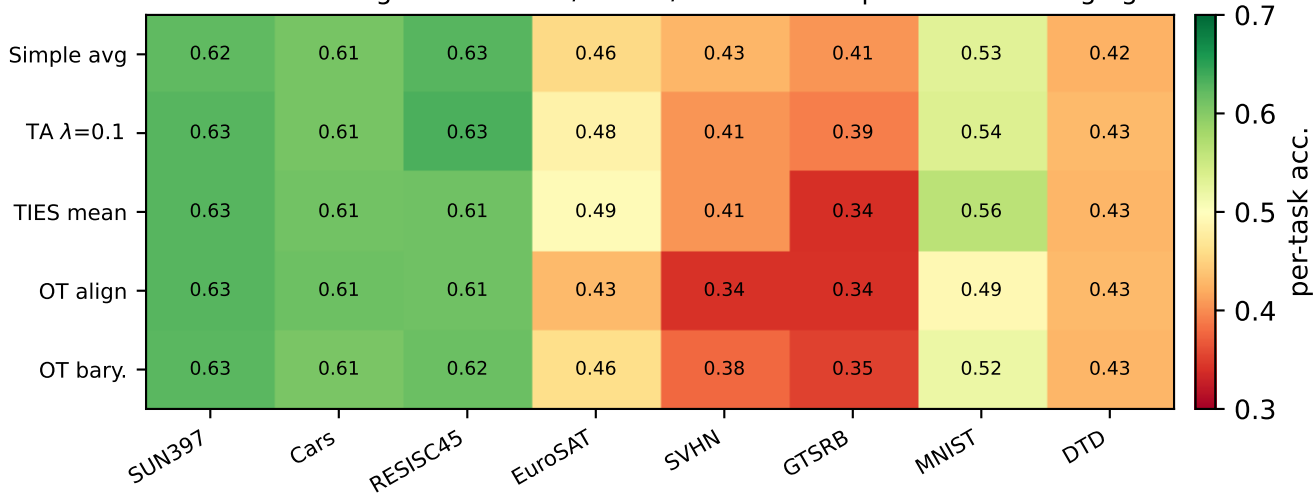
Interference signature: SVHN/GTSRB/EuroSAT collapse under averaging
