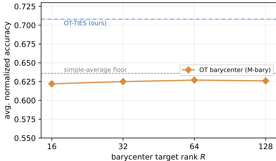
OT averaging plateaus at the floor regardless of rank (negative result)
