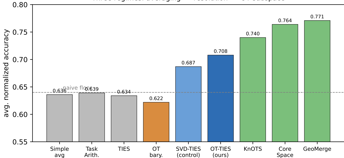
Three regimes: averaging \rightarrow resolution \rightarrow OT subspace
