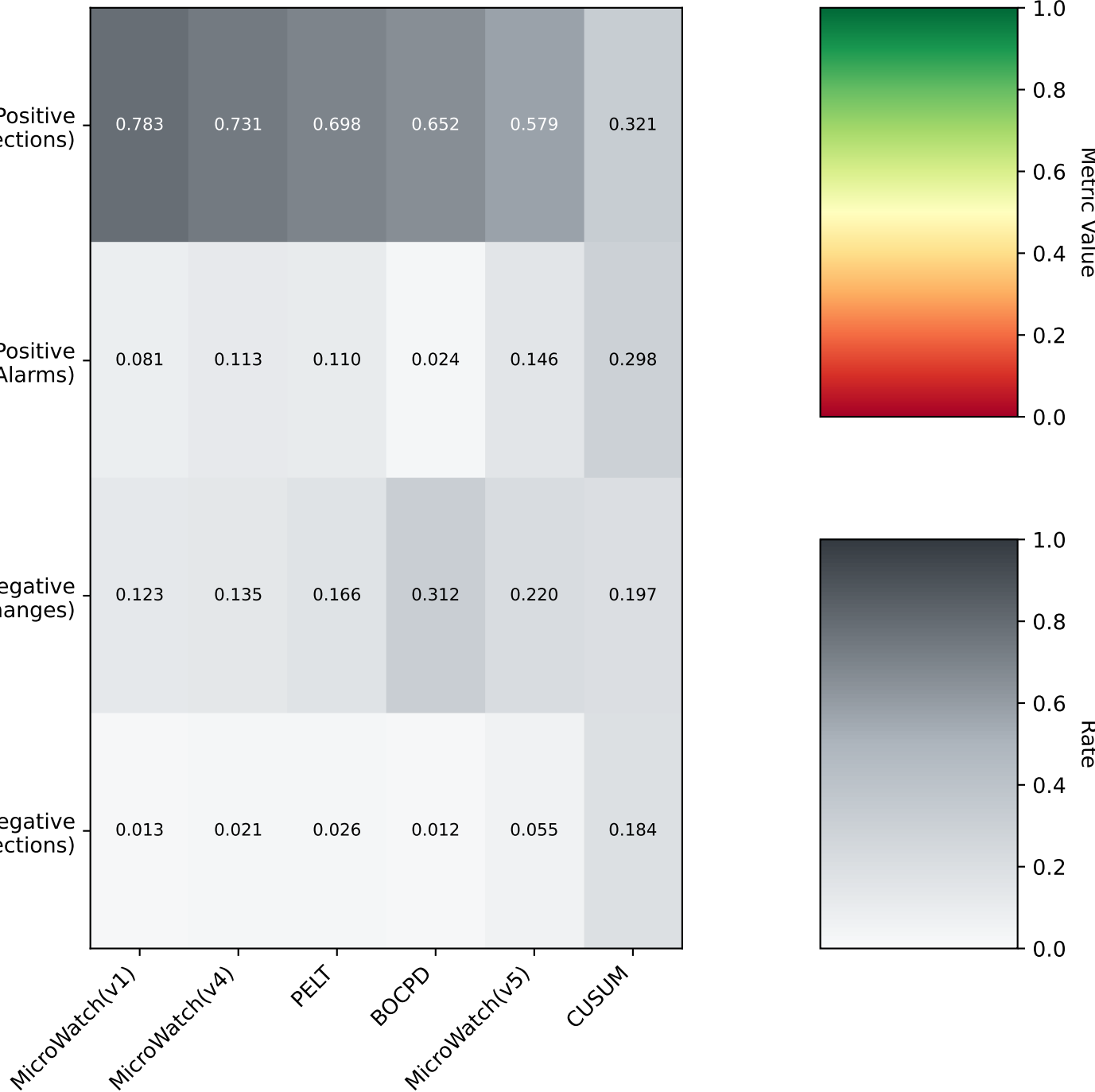
Detection Performance Breakdown (Derived from Precision & Recall)
