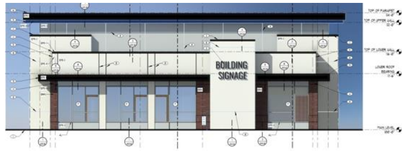
1 NORTH ELEVATION 10'-0"
