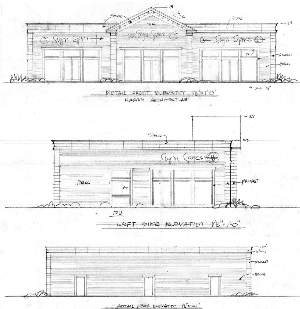
Retail Elevations
