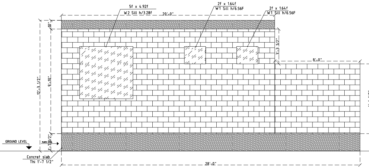
LEFT ELEVATION
