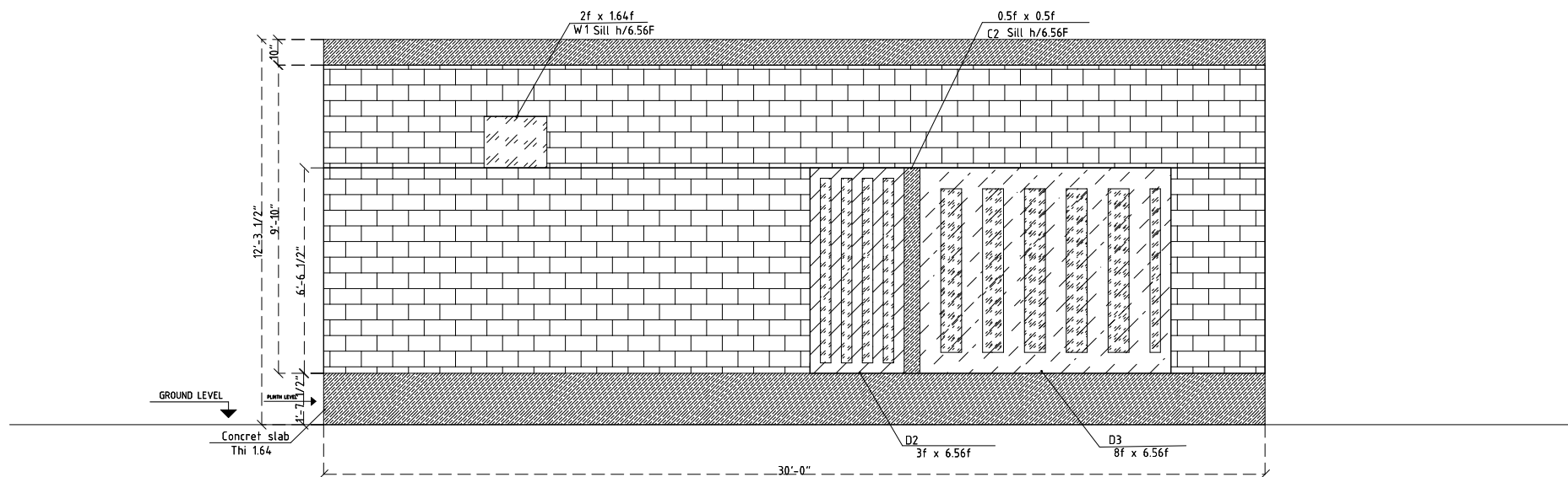
FRONT ELEVATION
