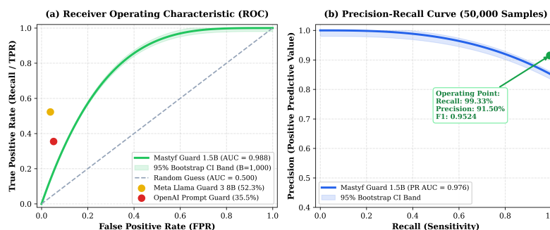
FIGURE 4: Massive 50,000-Sample Dual ROC and Precision-Recall Curves with 95% Bootstrap Confidence Bands.
