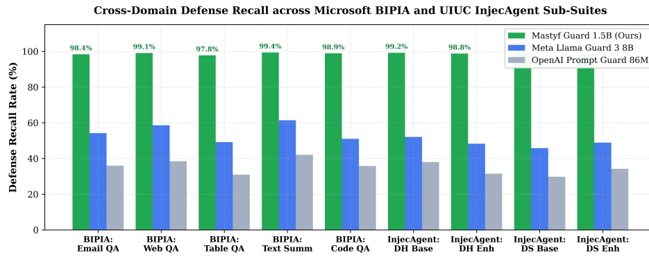
FIGURE 5: Granular Attack Defense Recall Across InjecAgent Sub-Tracks and Microsoft BIPIA Application Domains.
