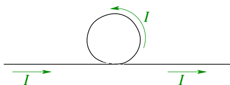
problem 3
