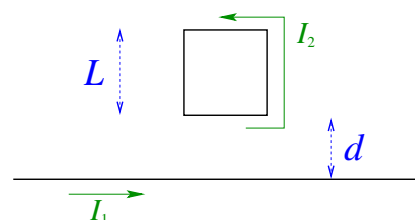
problem 4
