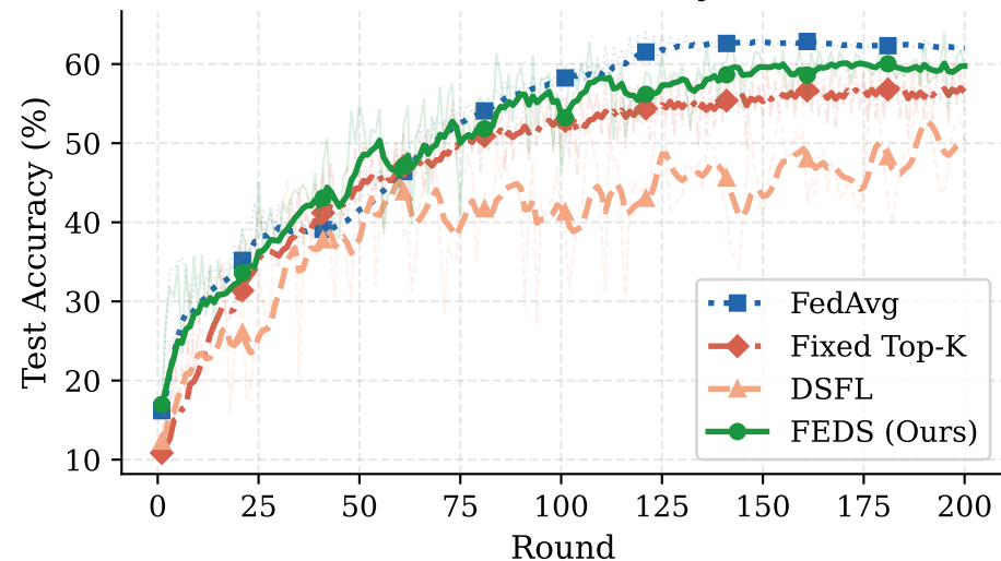
(a) Test Accuracy
