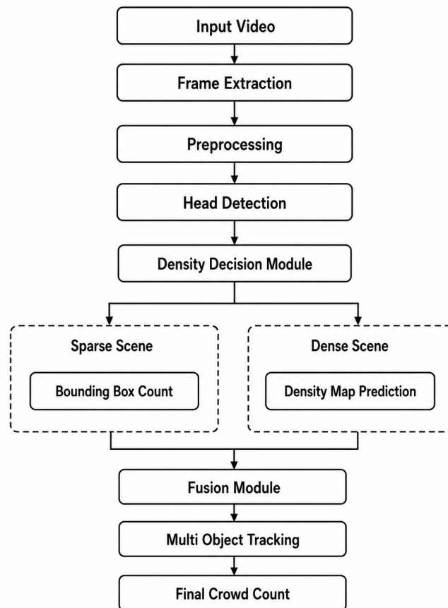
Figure 1: System Architecture
