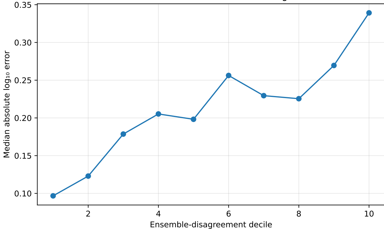
Error versus five-member XGBoost disagreement
