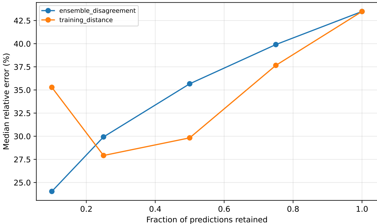
Selective prediction under source-held-out evaluation
