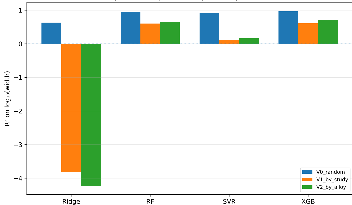
Melt-pool width: protocol-dependent performance
