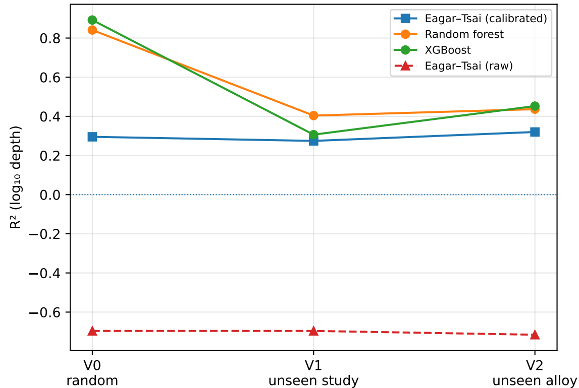
(a) Tree ensembles versus analytical physics
