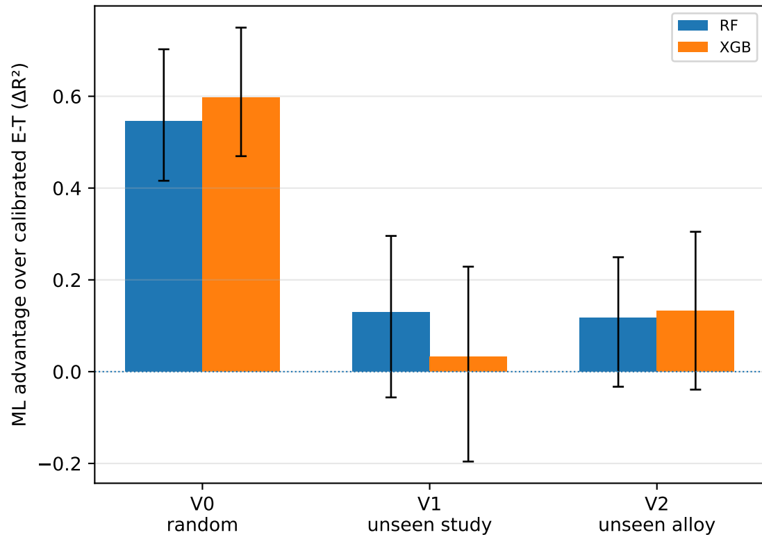
(b) Advantage depends on evaluation protocol
