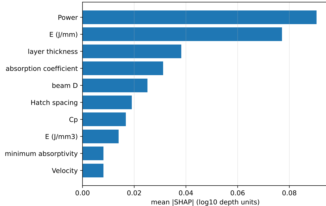
(a) Feature importance, unseen-study fold
