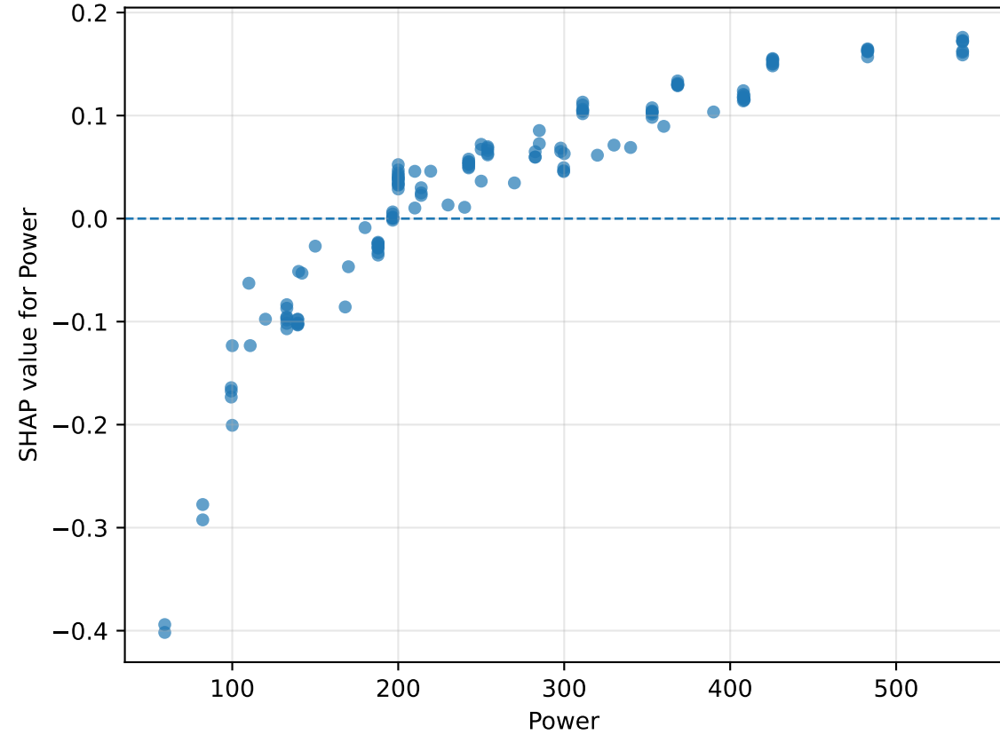
(b) Dependence: Power
