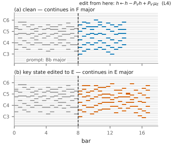
Fig. 1. The claim in one example (real model output, fixed sampling seed). We continue the same 8-bar Bb-major prompt (a) without an edit and (b) after we replace the key component of the layer-4 activations with the E-major class mean from bar 9 on. The input does not change , and the continuation follows the injected value. Shading marks the scale of the key in force.
