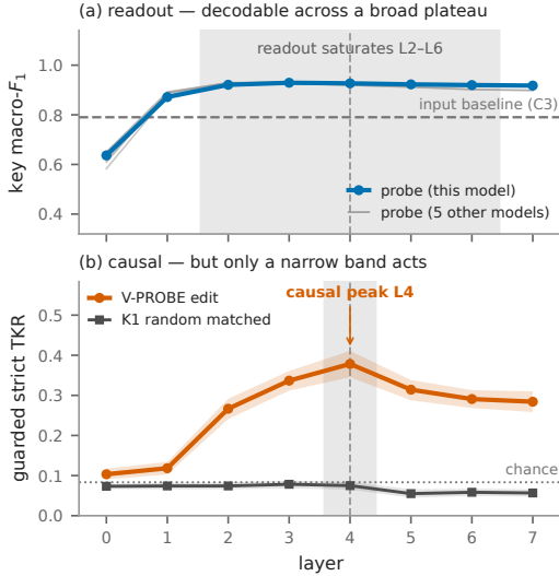
Fig. 3. (a) Probe macro- F_1 per layer for all six models (thin lines; seed 0 highlighted). We can read the key across a broad band. (b) Causal effect of the edit against the K1 matched control (bands: prompt-level bootstrap 95% CI). The edit changes the output only in a narrow band. These are selection-phase data; the confirmatory run fixes L4 and repeats no search.
