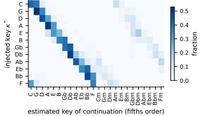
Fig. 4. Specificity [s0]: distribution of the continuation’s estimated key (columns, fifths order) per injected key (rows), V-PROBE edit at L4.
