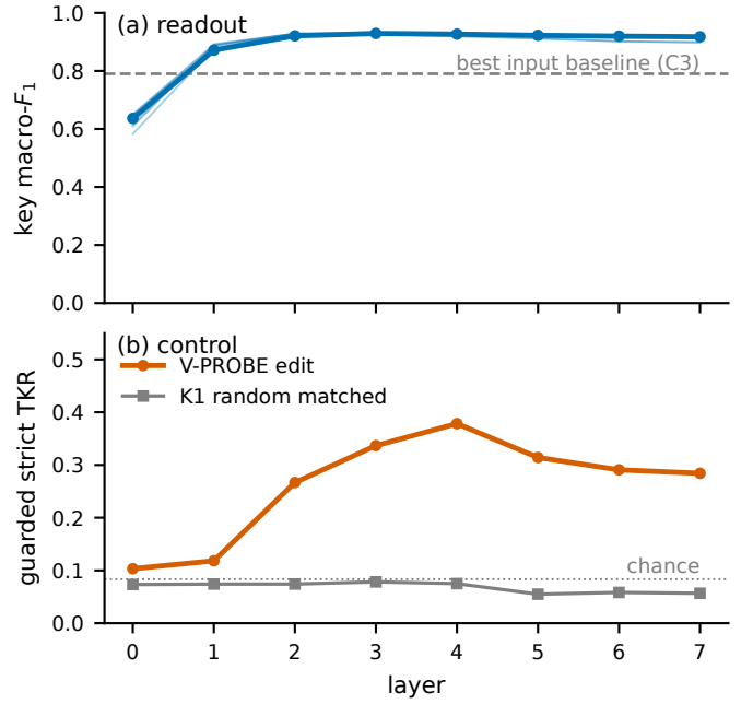
Fig. 1. The key is read and used in the same middle layers. (a) Linear-probe macro- F_1 per layer for all six M-CTRL models (thin lines; R-Aug seed 0 highlighted) against the best input baseline. (b) Causal effect [s0]: guarded strict TKR of the V-PROBE edit vs. the K1 matched random control.
