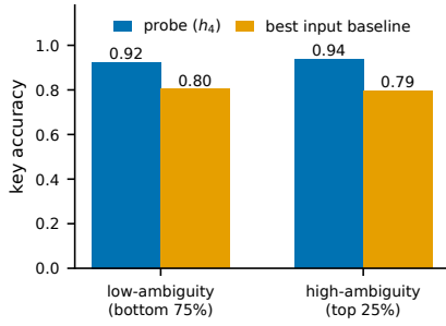
Fig. 2. Probe vs. input baseline by ambiguity stratum (L4, [s0] model): the probe’s margin is largest where surface statistics are least informative.
