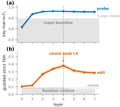
Fig. 3. (a) Probe macro- F_1 per layer, all six models; gray marks the best input baseline. The key is readable across a broad band. (b) Causal effect of the edit (band: prompt-level bootstrap 95% CI); gray reaches to the K1 control’s CI ceiling. Only a narrow band acts. Selection-phase data; the confirmatory run fixes L4.
