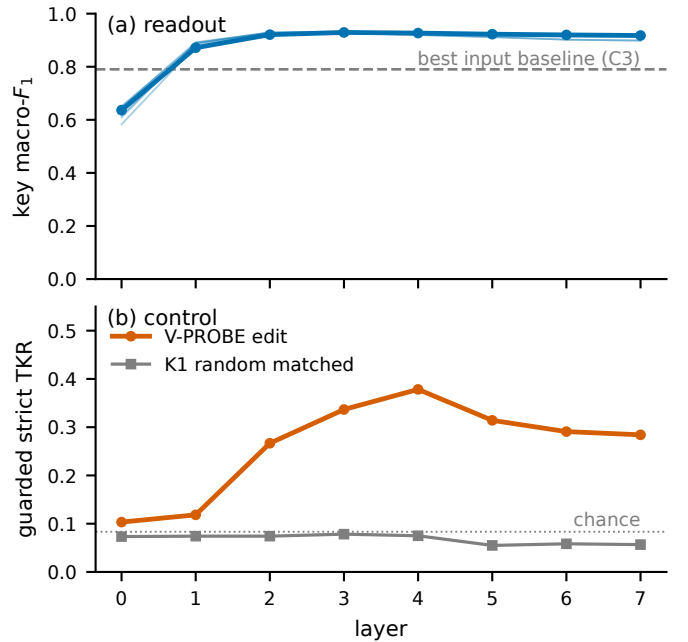
Fig. 2. The key is read and used in the same middle layers. (a) Linear-probe macro- F_1 per layer for all six M-CTRL models (thin lines; R-Aug seed 0 highlighted) against the best input baseline. (b) Causal effect [s0]: guarded strict TKR of the V-PROBE edit vs. the K1 matched random control.
