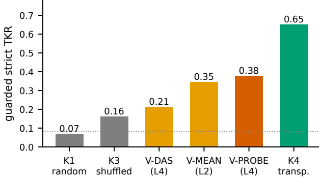
Fig. 6. Guarded strict TKR across conditions [s0] (dotted line: chance 1/12 ): the probe-subspace edit at its best layer moves the composed key at 5.6\times the matched random control and reaches 58% of the transposed-prompt behavioral reference.
