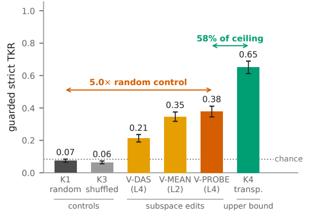
Fig. 3. Guarded strict TKR by condition: the continuation lands exactly on the injected key and stays inside the frozen musicality budget. Chance = 1/12. Bars: prompt-level bootstrap 95% CI.
