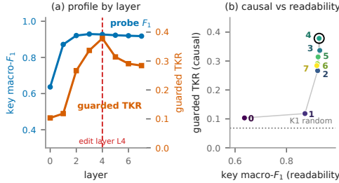
Fig. 3. (a) Probe macro- F_1 (blue, left axis) and guarded TKR of the edit (vermillion, right axis) per layer; the dashed line marks the frozen edit layer. (b) Causal effect against readability, one point per layer, numbered by depth; the frozen layer is circled and the dotted line is the K1 random control. Readability clusters while causal effect spans an order of magnitude. Selection-phase data, seed 0; per-seed variants in the supplementary.
