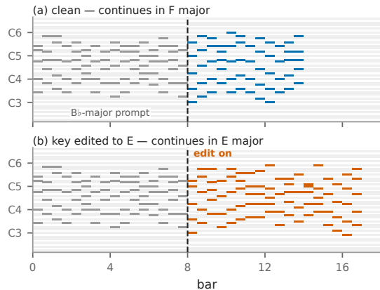
Fig. 1. The claim in one example (real model output, one fixed sampling seed). We continue the same 8-bar Bb-major prompt (a) without an edit and (b) after we write the E-major key part into the layer-4 activations from bar 9 on. The prompt is identical in both panels, and the continuation follows the key we install. In (a) the unedited continuation moves to the dominant, an ordinary move; in (b) it moves to E major, which is not. Shading marks the scale of the key in force.
