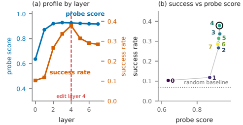
Fig. 3. (a) The probe score (blue, left axis) and the success rate of the edit (orange, right axis) at each layer; the dashed line marks the edit layer that the final test fixes. (b) The same two numbers plotted against each other, one point per layer, numbered by depth; the black circle marks the final-test layer, and the dotted line is the random baseline. The key reads almost equally well from layers 2–7, yet the edit acts only in the middle; the probe score is the macro- F_1 of Section V-A. Search-stage data, seed 0.
