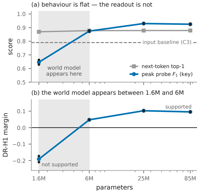
Fig. 5. Behavioral equivalence, representational dissociation. Across a 50\times capacity range next-token accuracy is flat, but the key readout is not: below \sim 6M the probe cannot beat the input baseline and the pre-registered DR-H1 margin is negative. Dots: seeds.
