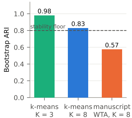
c Only the small partition reproduces
