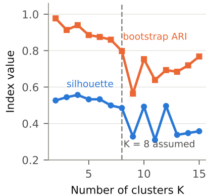
a No index selects eight clusters
