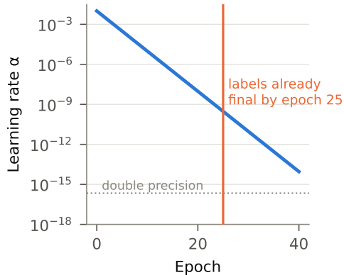
b Training freezes almost at once
