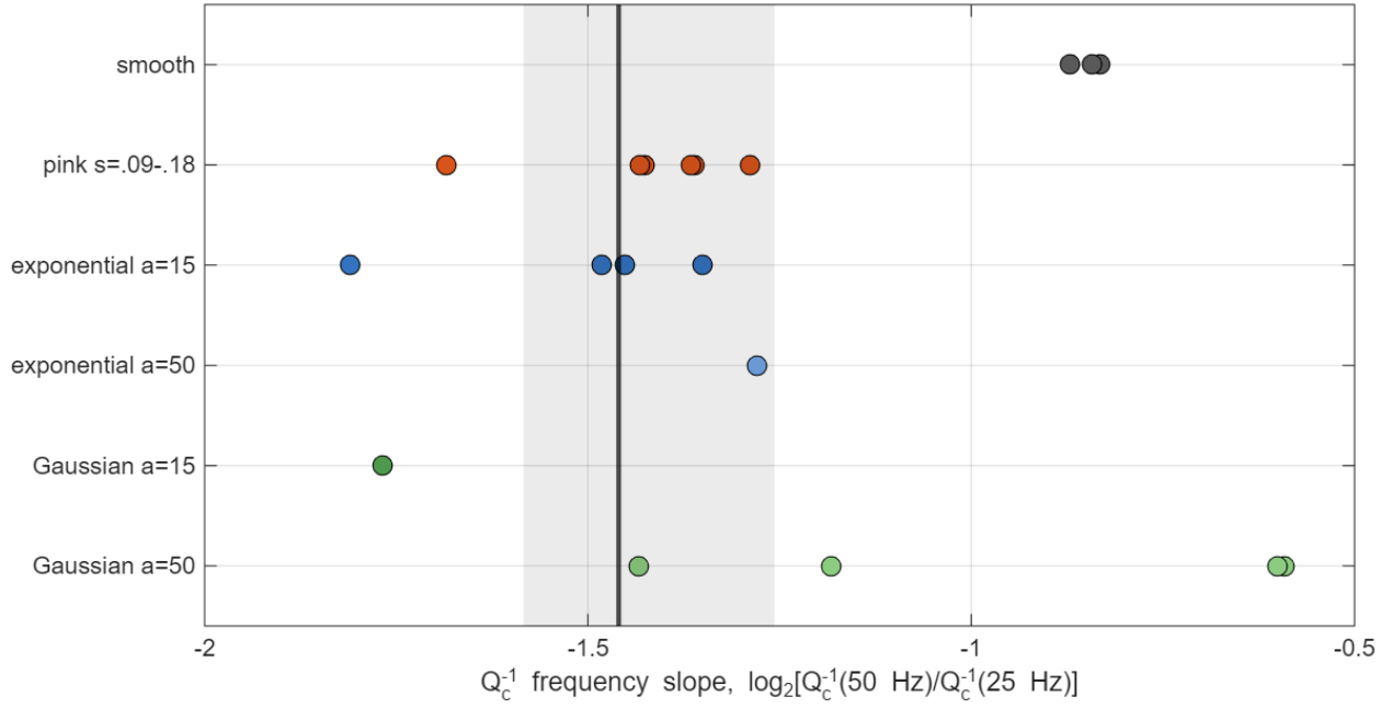
Figure S8. Q_c^{-1} frequency slope \log_2[Q_c^{-1}(50 \text{ Hz})/Q_c^{-1}(25 \text{ Hz})] at sensor A, FORGE (black line, grey 95 % bootstrap band) and simulated media (dots). A finite-window diagnostic: data and synthetics are measured identically, but the absolute values are not medium properties.
