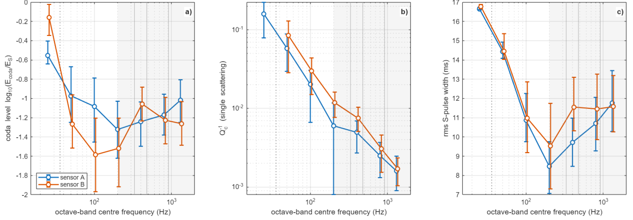
Figure S7. FORGE coda measures in seven octave bands (25 Hz to 1.3 kHz): a) coda level, b) single-scattering Q_c^{-1} (finite-window diagnostic; at 25 Hz the window spans one to three periods), c) rms S-pulse width. Median and interquartile range for sensors A and B. Shaded (> 200 Hz): affected by the resonances.
