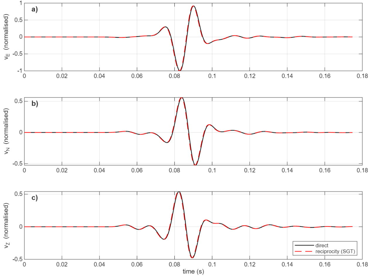
Figure S1. Reciprocity validation in a heterogeneous VTI pink-noise medium ( \sigma = 0.045 , \varepsilon = 0.05 , \delta = 0.02 , \gamma = 0.05 ). a–c) East, north and vertical velocity at a sensor from a direct double-couple simulation (black) and from the strain-Green's-tensor reciprocity synthetic (red dashed). Correlation and amplitude ratio are 0.995.
