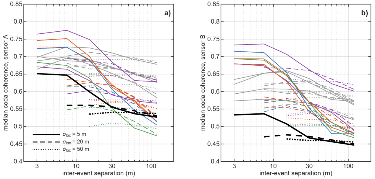
Figure S10. Location stress test of the inter-event coda coherence (window S + 40 to S + 100 ms): binned medians after perturbing the hypocentres used for binning by isotropic Gaussian errors of 5 m (solid), 20 m (dashed) and 50 m (dotted), for FORGE (black, thick) and the media (colours as in main-text Fig. 7). a) Sensor A. b) Sensor B. Large errors flatten the curves of data and media alike; the levels at \geq 20 m separation are preserved.
