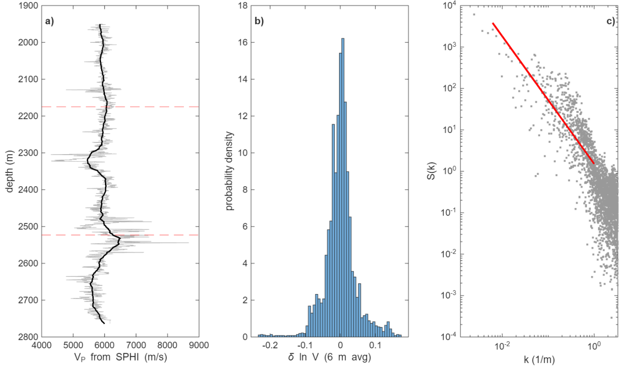
Figure S2. The 56-32 sonic log. a) Sonic-derived V_p (grey) and its 50-m block average (black); dashed lines mark the depths of sensors A and B. b) Distribution of the detrended, 6-m-averaged \delta \ln V . c) Periodogram of \delta \ln V with a power-law fit over 1–200 m. Slope uncertainty is given in Table S15 and main-text Fig. 9.
