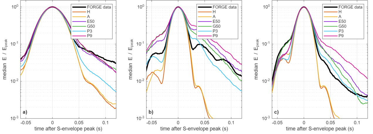
Figure S4. Median S-coda envelopes aligned on the S peak and normalized by it: a) sensor A, 20–40 Hz; b) sensor A, 40–80 Hz; c) sensor B, 40–80 Hz. Black: FORGE; H homogeneous; A VTI; E50/G50 exponential/Gaussian ( a = 50 m, \sigma = 0.13 ); P3/P9 pink ( \sigma = 0.09/0.18 ).
