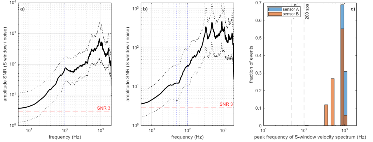
Figure S6. a, b) Median (solid) and interquartile range (dotted) of the S-window amplitude SNR spectrum for sensors A and B; horizontal line at SNR = 3. c) Peak frequency of the S-window velocity spectrum for all events. The clustering near 330, 480 and 920 Hz indicates tool or coupling resonances; the share of recorded velocity energy above 100 Hz is therefore not a source or path property.
