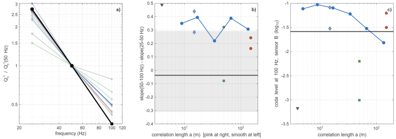
Figure S9. Exploratory high-frequency series (2.5-m grid, sensor B, reduced volume, noise-free synthetics, \sigma = 0.13 ). a) Q_c^{-1} normalized at 50 Hz from the 25–50 Hz (sensor A, 5-m grid) and 50–100 Hz (sensor B, 2.5-m grid) slopes. b) Curvature of Q_c^{-1} versus correlation length. c) Coda level at 100 Hz versus correlation length; black line: FORGE. Grid, domain, sensor and event subset change together between the two octaves, so the comparison is not a pure frequency effect.
