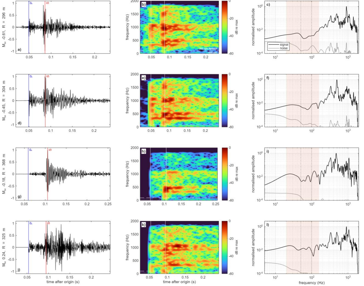
Figure S5. Four example events (magnitude -0.61 to +0.24 ) at sensor B, 4 kHz. a, d, g, j) Horizontal velocity ( > 5 Hz) with P (blue) and S (red). b, e, h, k) Spectrograms to 2 kHz on a common dB scale relative to each event's maximum; white dashed and dotted lines mark 100 and 50 Hz, the Nyquist frequencies of 200 and 100 sample/s recording. c, f, i, l) S-window spectrum (black) and pre-event noise (grey); shaded: FD analysis band.
