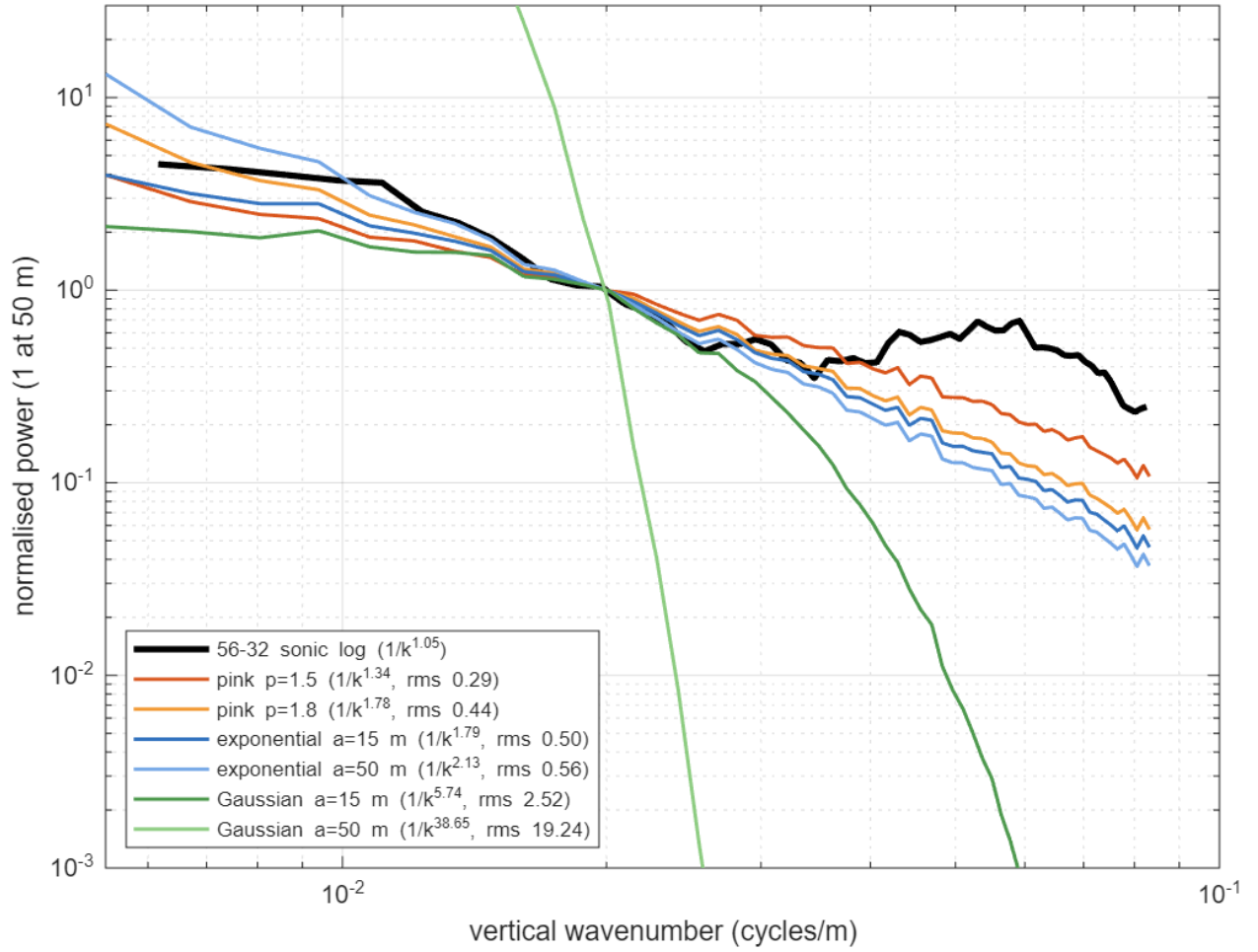
Fig. S11 Vertical fluctuation spectra of the 56-32 sonic log (black) and of the model media over 12–200 m, normalised at 50 m. The rms log difference in the legend is a descriptive distance, not a likelihood.
