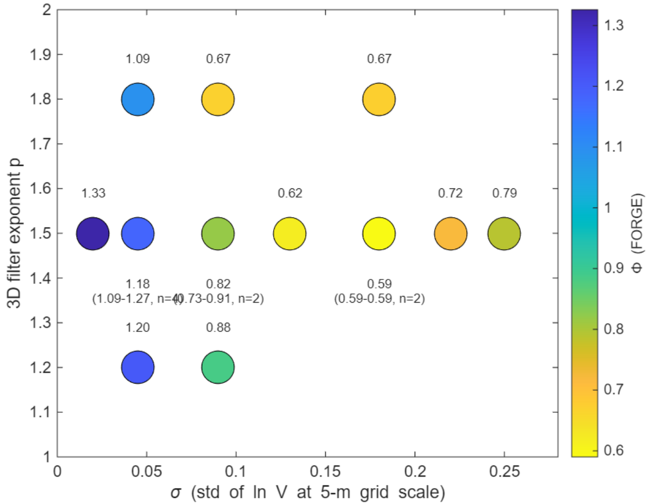
Fig. S12 Original \Phi over the pink-family parameters ( \sigma , p ) for FORGE; mean and range where several realisations exist. \sigma = 0.22 and 0.25 have fewer than five grid points per minimum S wavelength at 80 Hz.
