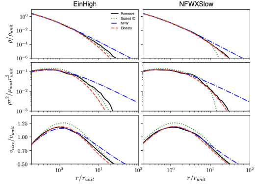
Figure 2. This is a figure from Drakos et al. (2019) which illustrates the methodology intended to pursue to analyze the DM halo remnant after a major merger. The diagram shows the density profile and the circular velocity profile which are both plotted as a function of radius. The remnant is then compared to the theoretical models such as NFW, Einasto, and scaled initial conditions. This comparison is intended to convey how accurate the analytic profiles match the simulated merger remnant.
