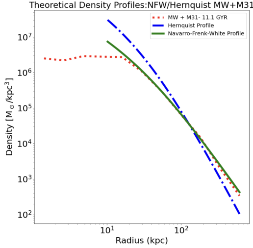
Figure 4. This plot is the theoretical density profiles of the Dark Matter halo compared with the simulated merged Dark Matter halo, which is represented by the red dotted line. The Hernquist profile is shown as the dashed blue line, and the Navarro-Frenk-White profile is the solid green line. The x-axis represents the radial distance from the center in kpc, while the y-axis shows the DM density in M_{\odot}/kpc^3 . I used a scale radius of 28 for both profiles, Mhalo is 3.895 \times 10^9 M_{\odot} , \rho_0 = 5.0469 \times 10^6 M_{\odot} / kpc^3 and r is the average radial distance from center. The figure reveals the NFW profile aligns remarkably better with the simulated density distribution, especially at larger radii. It best describes the structure of the post merger Dark matter remnant.
