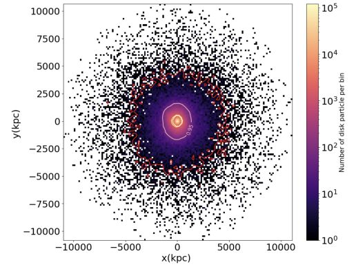
Figure 5. A face on 2D contour plot of the final merged Dark Matter halo. The x-axis and y-axis represent the particle positions in kpc. The color bar is the number of particles per bin on a log scale. The red contour lines represent where the distribution is symmetrical and where most of the Dark Matter is concentrated. This figure shows an overview of how Dark Matter particles settle after a major merger, reflecting a heavily dense center/core.
