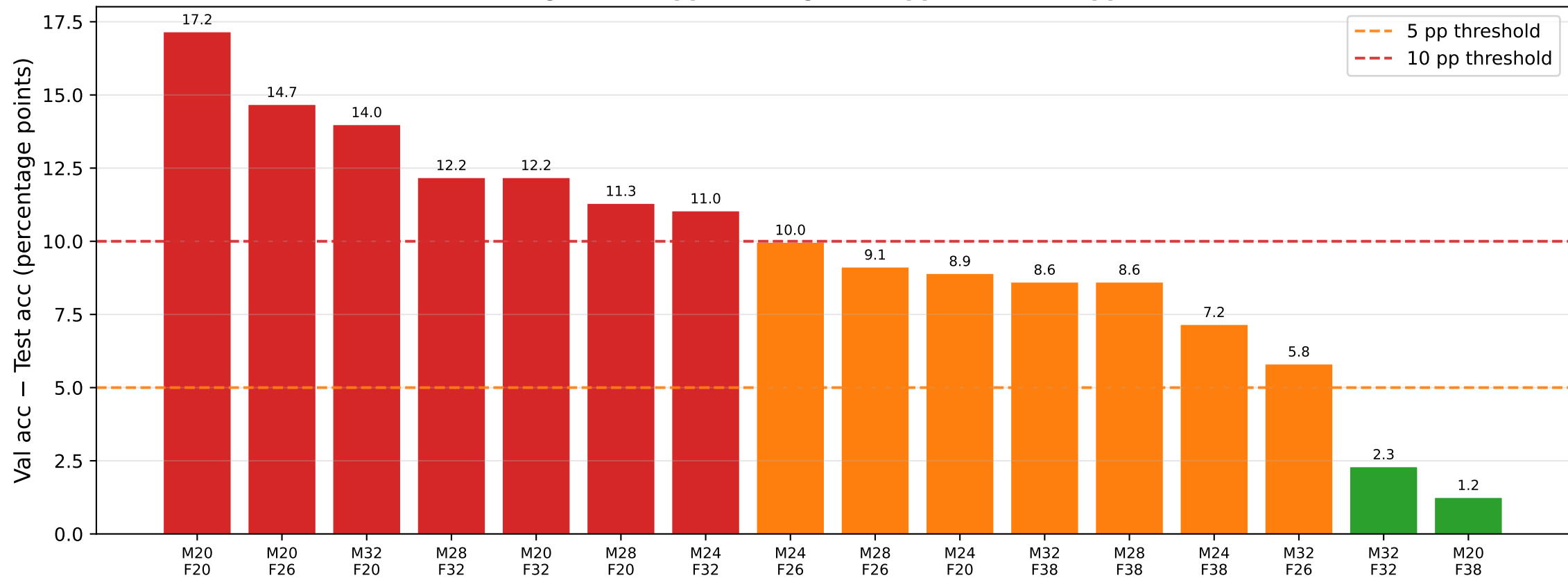
Generalisation gap per configuration (Val – Test) green < 5 pp · orange 5-10 pp · red > 10 pp
