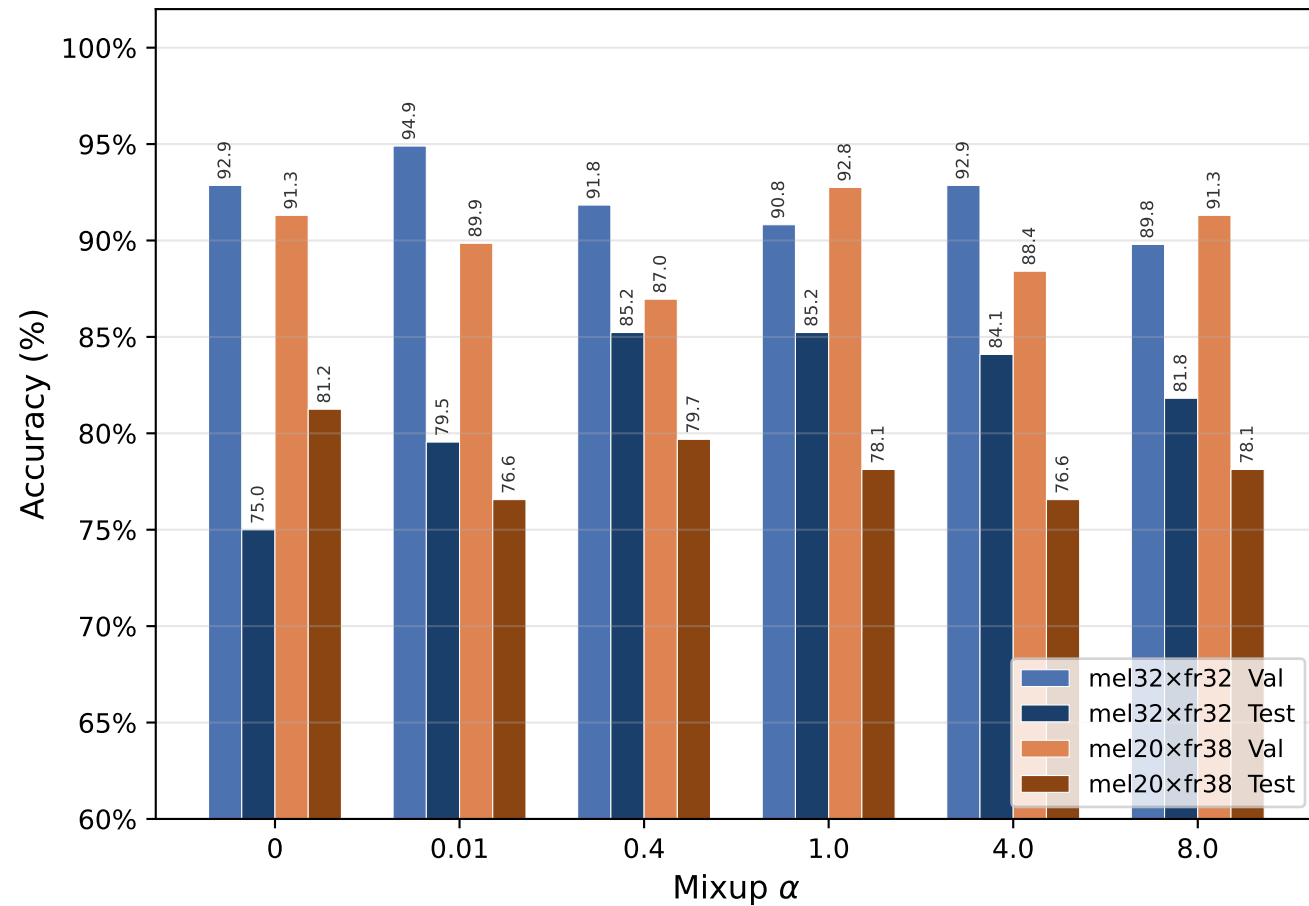
Accuracy vs Mixup \alpha (dropout = 0.25) mel32×fr32 vs mel20×fr38
