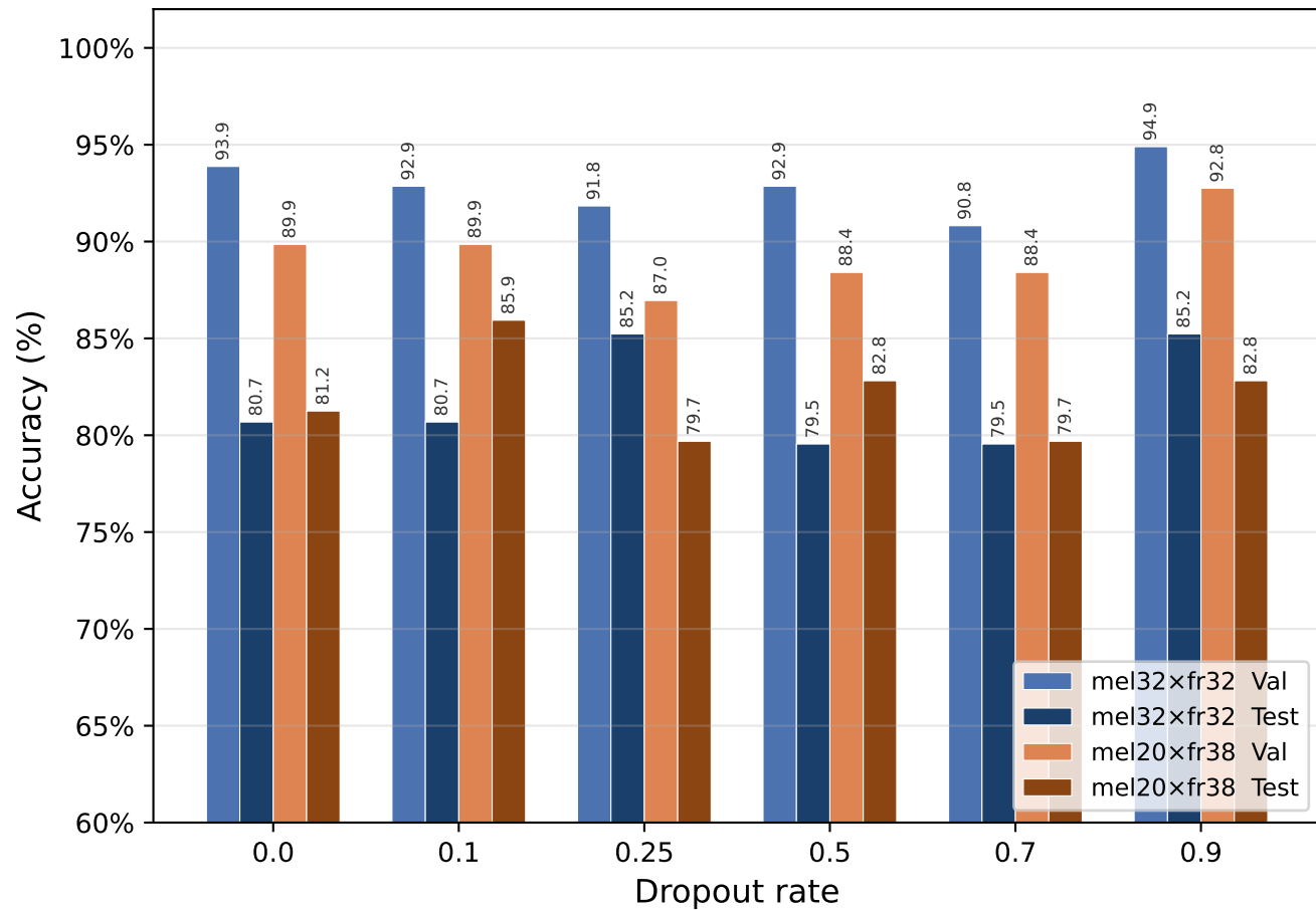
Accuracy vs Dropout (mixup \alpha = 0.4 ) mel32×fr32 vs mel20×fr38
